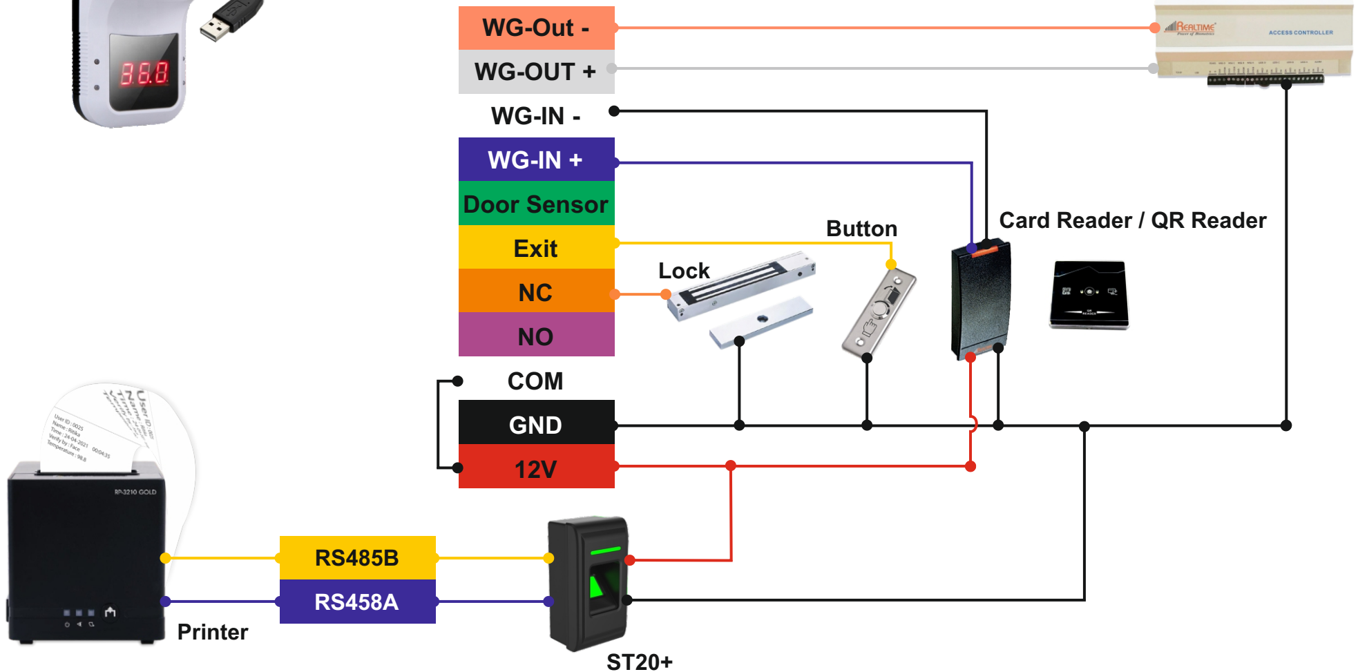
External Controller
